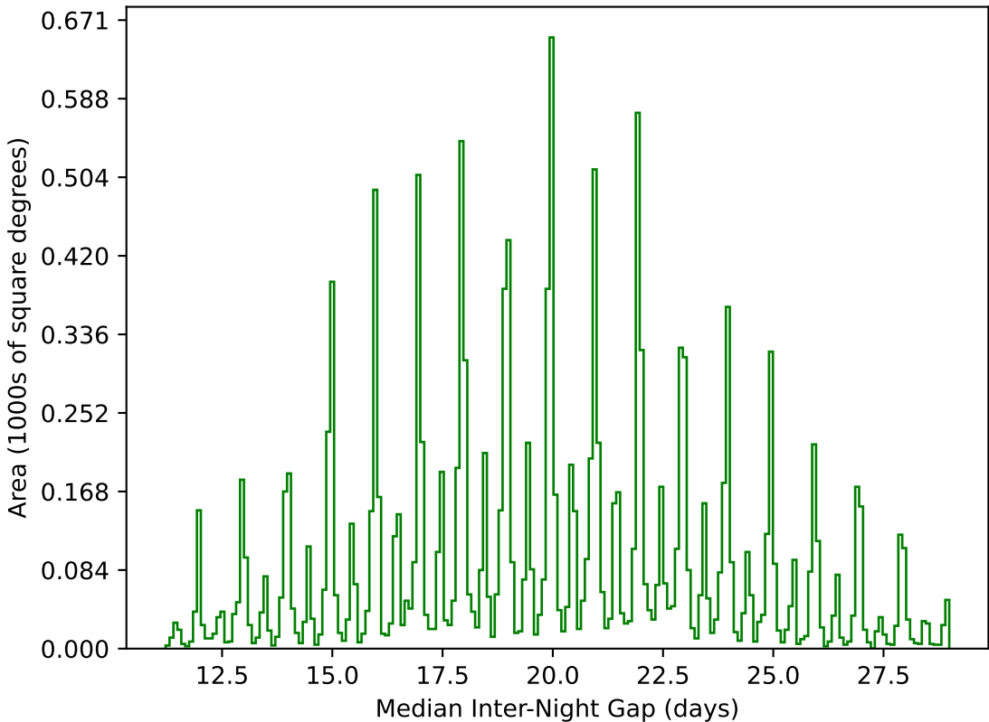
too_elab_r128_d3_gz_v3.4_10yrs WFD g band: Median Inter-Night Gap
