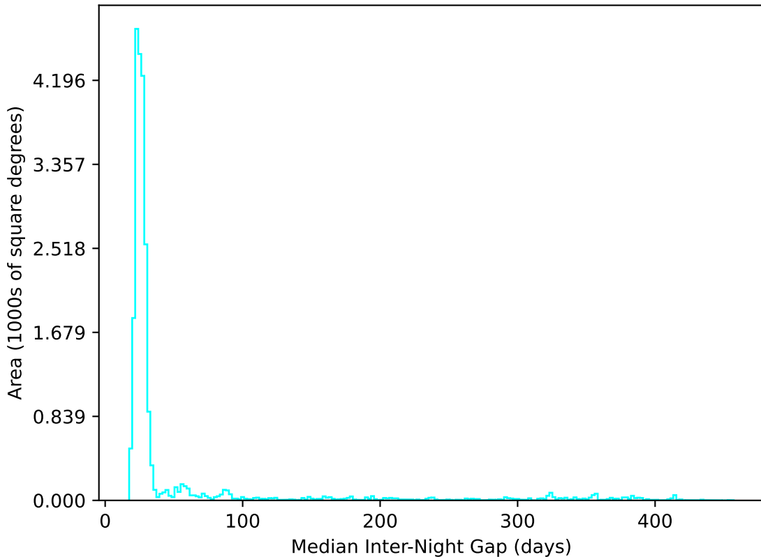
too_elab_r128_d3_gz_v3.4_10yrs All sky u band: Median Inter-Night Gap
