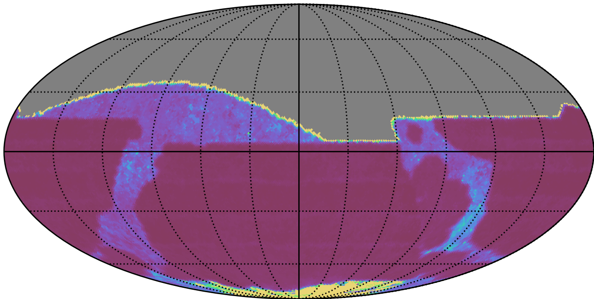
too_elab_r128_d3_gz_v3.4_10yrs All sky r band: Median Inter-Night Gap
