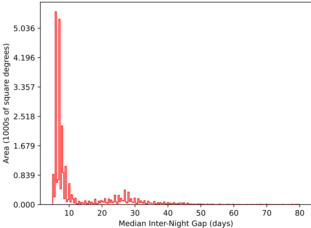
too_elab_r128_d3_gz_v3.4_10yrs All sky i band: Median Inter-Night Gap
