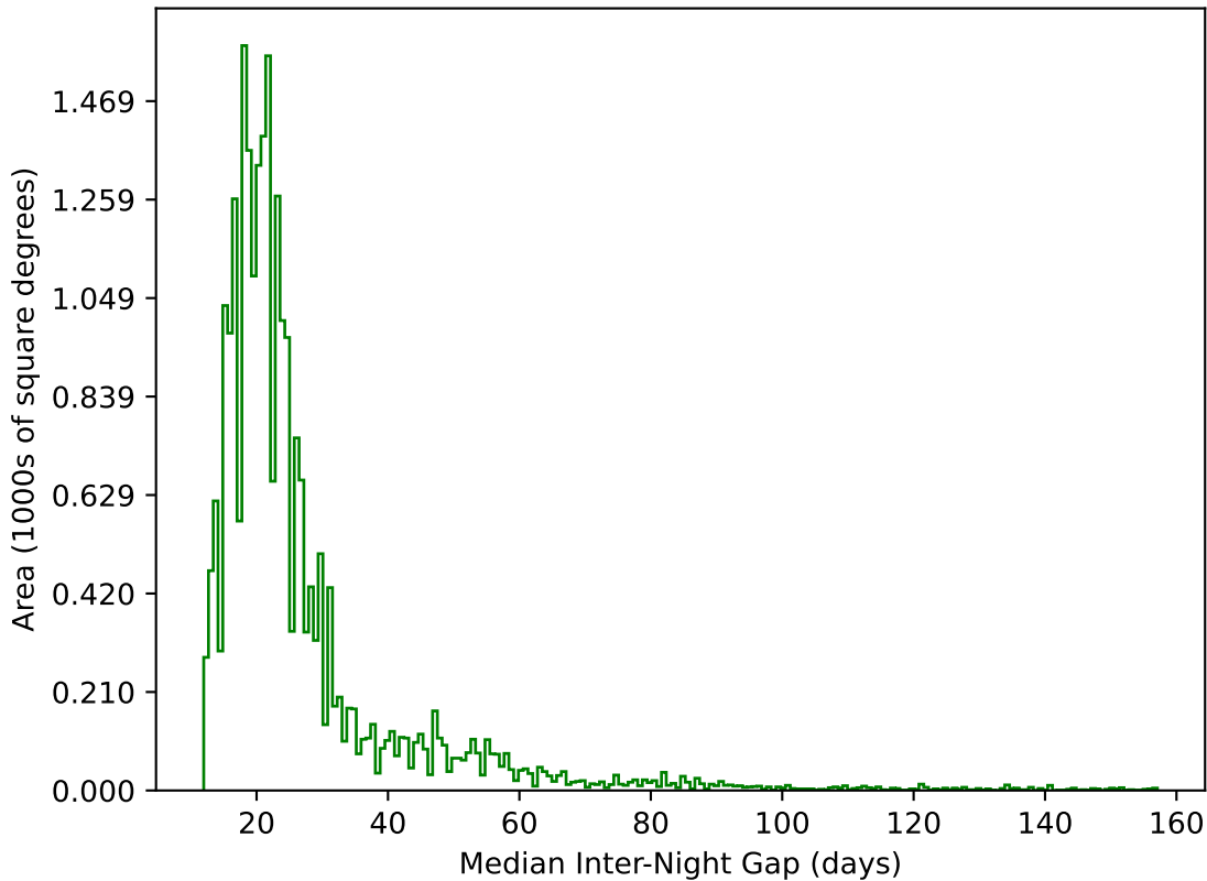
too_elab_r128_d3_gz_v3.4_10yrs All sky g band: Median Inter-Night Gap
