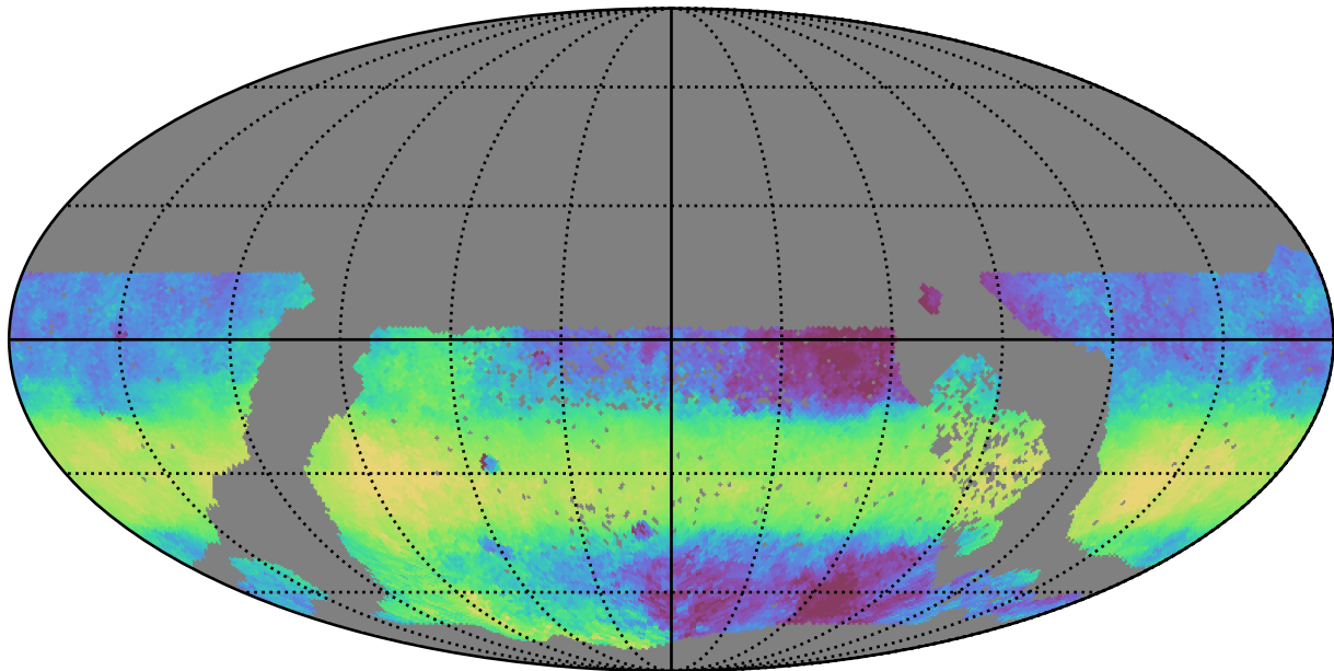
too_elab_r128_d3_gz_v3.4_10yrs WFD y band: Median HA
