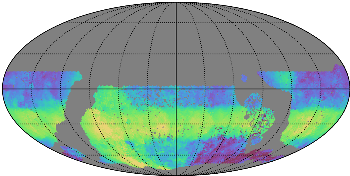
too_elab_r128_d3_gz_v3.4_10yrs WFD u band: Median HA
