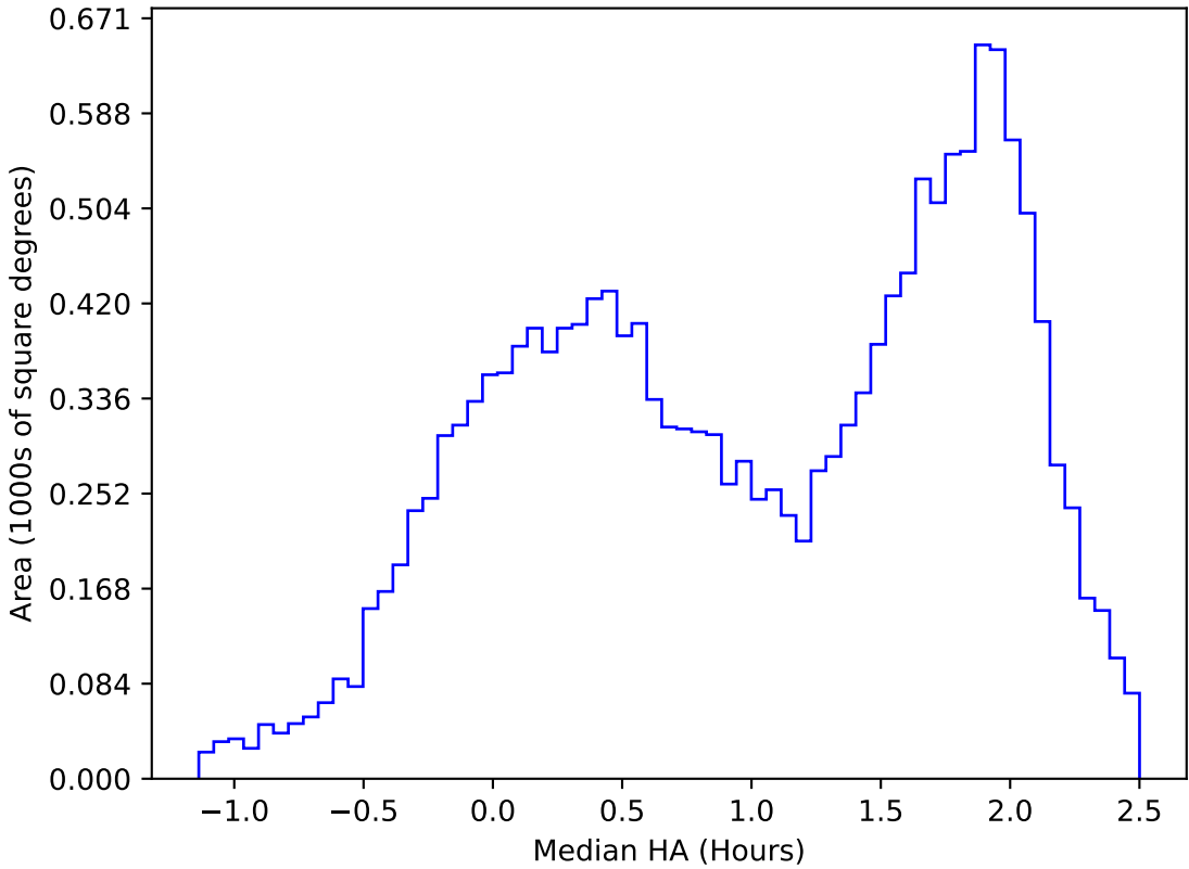
too_elab_r128_d3_gz_v3.4_10yrs WFD u band: Median HA
