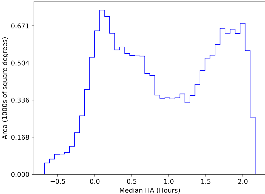
too_elab_r128_d3_gz_v3.4_10yrs WFD r band: Median HA
