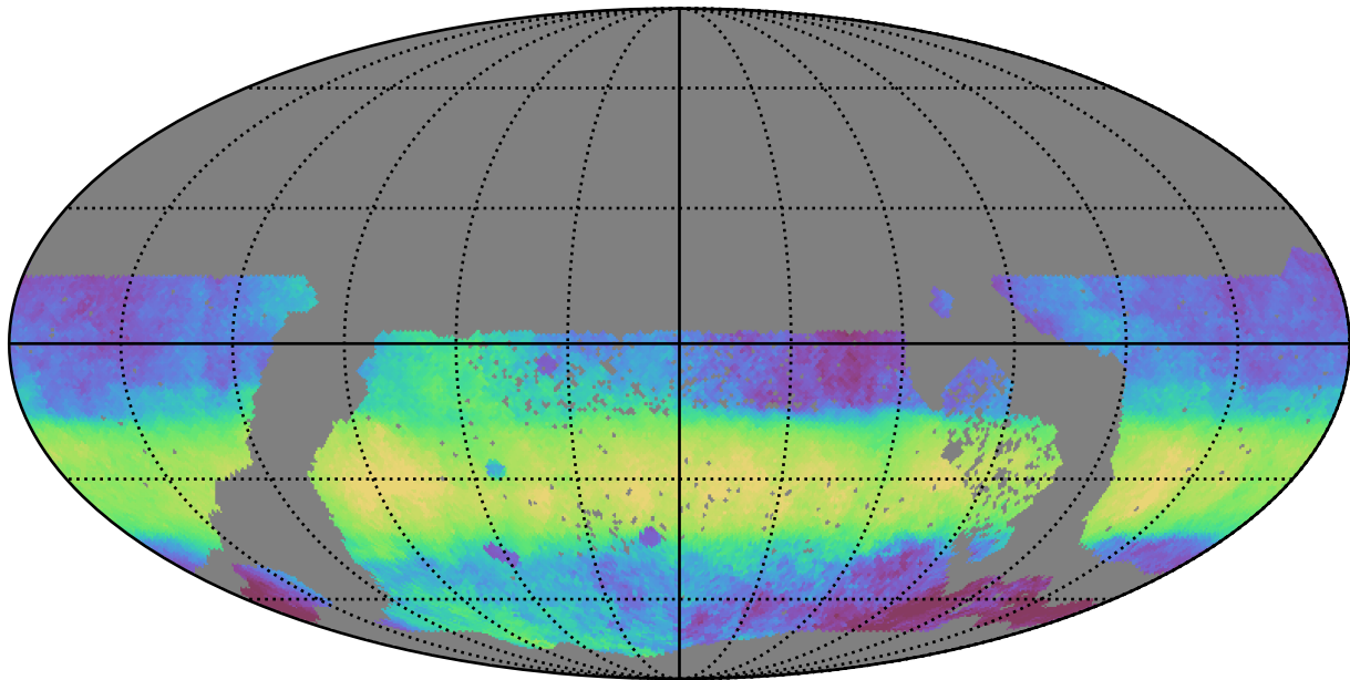
too_elab_r128_d3_gz_v3.4_10yrs WFD i band: Median HA
