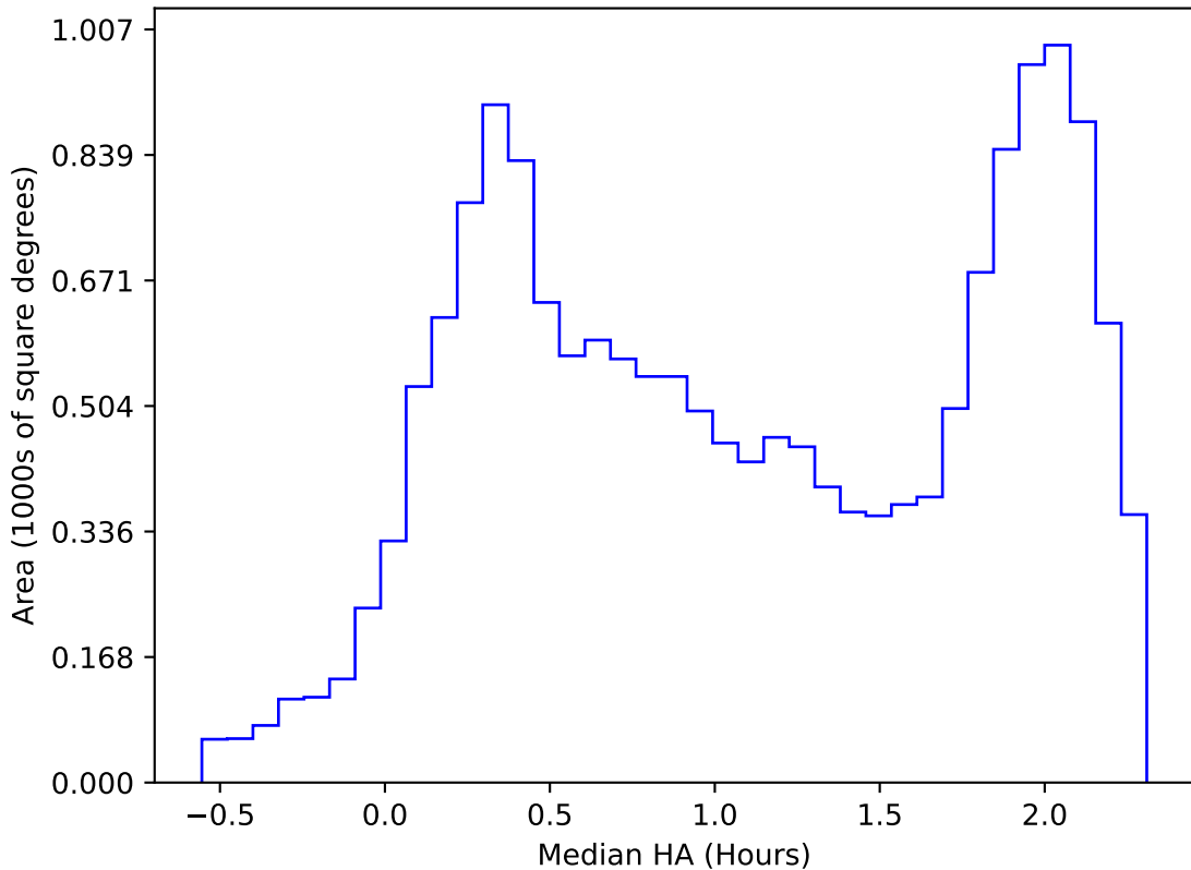
too_elab_r128_d3_gz_v3.4_10yrs WFD i band: Median HA
