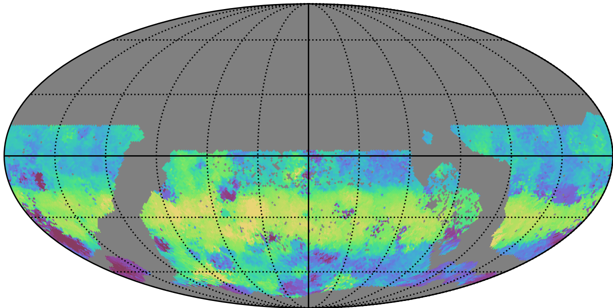
too_elab_r128_d3_gz_v3.4_10yrs WFD g band: Median HA
