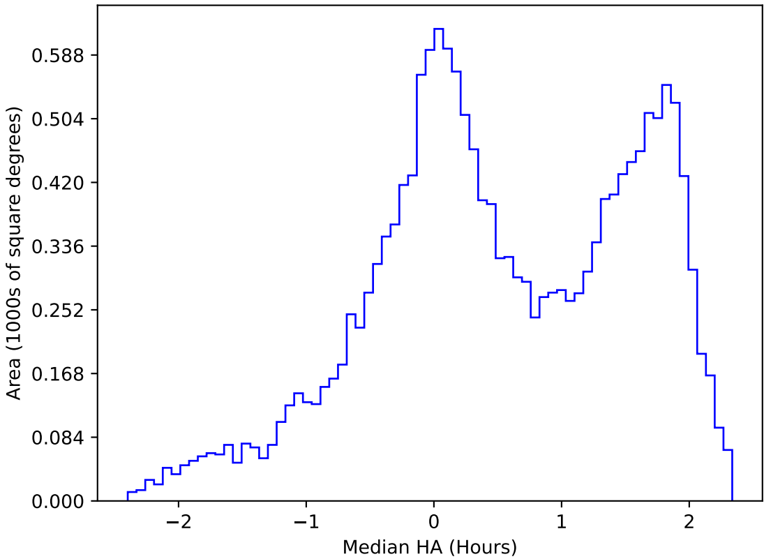
too_elab_r128_d3_gz_v3.4_10yrs WFD g band: Median HA
