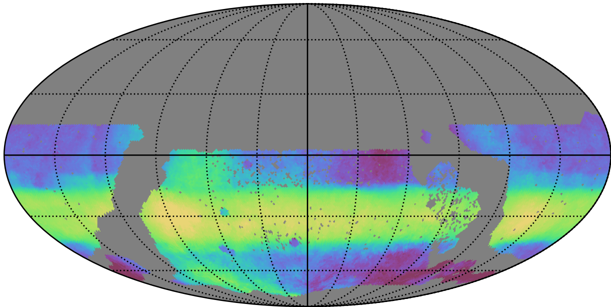
too_elab_r128_d3_gz_v3.4_10yrs WFD all bands: Median HA
