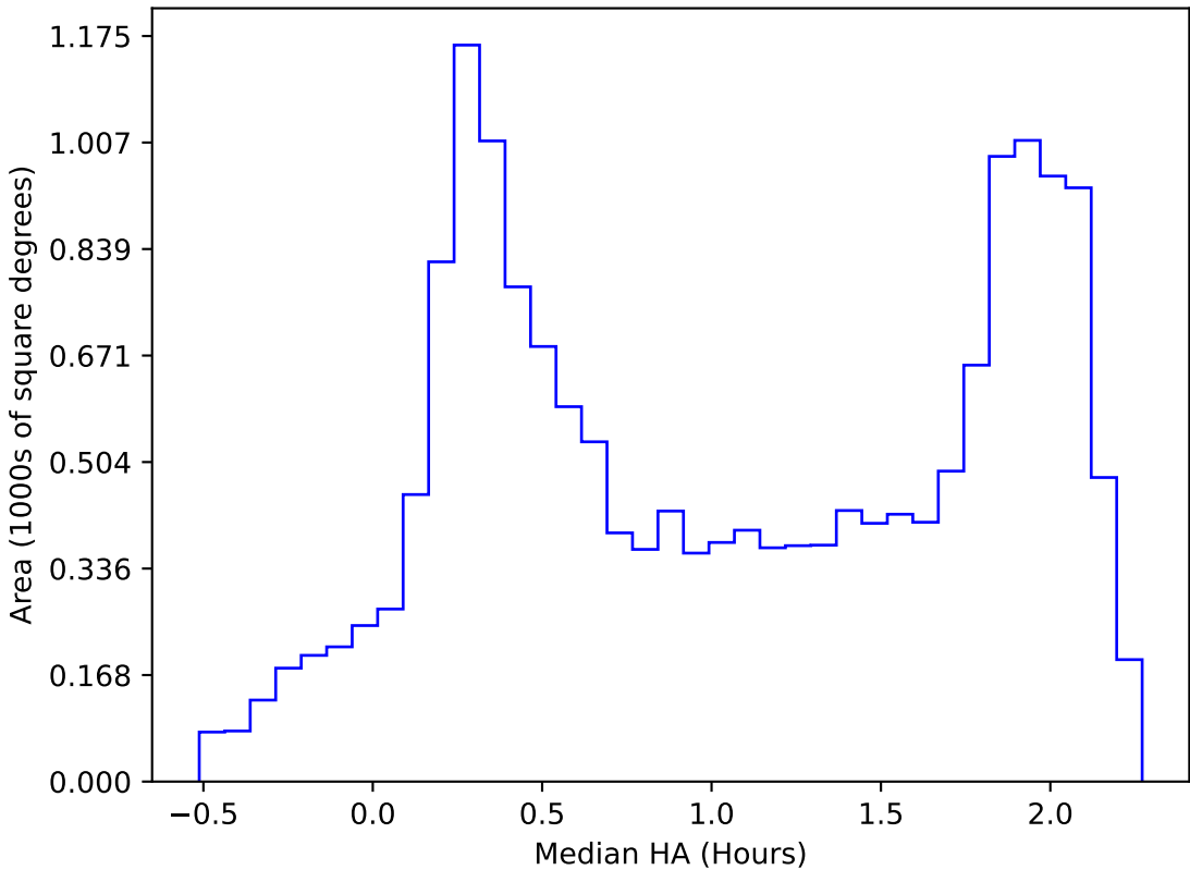
too_elab_r128_d3_gz_v3.4_10yrs WFD all bands: Median HA
