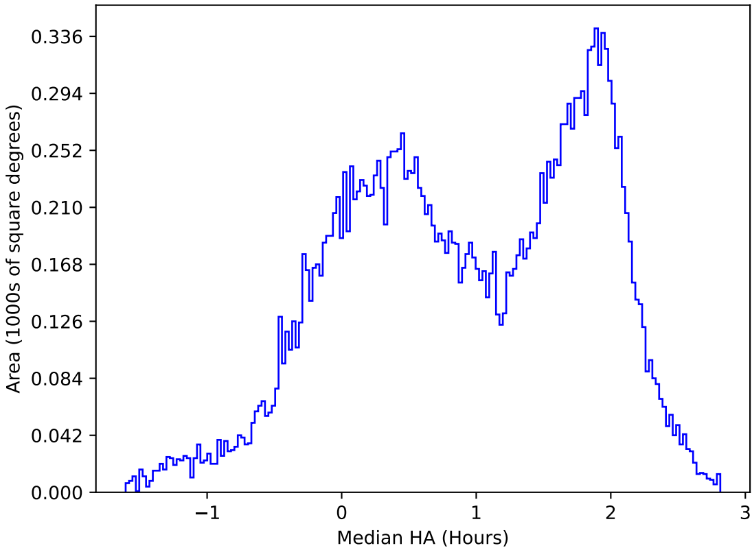
too_elab_r128_d3_gz_v3.4_10yrs All sky u band: Median HA
