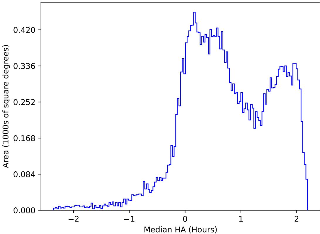
too_elab_r128_d3_gz_v3.4_10yrs All sky r band: Median HA
