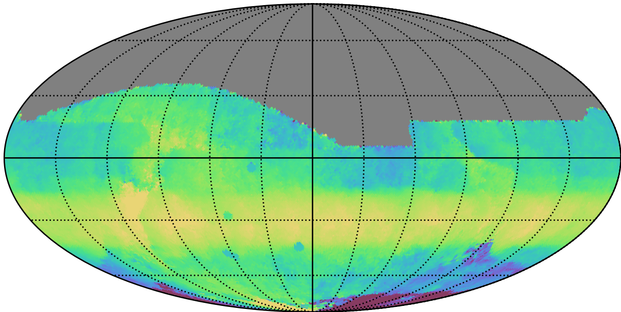
too_elab_r128_d3_gz_v3.4_10yrs All sky i band: Median HA
