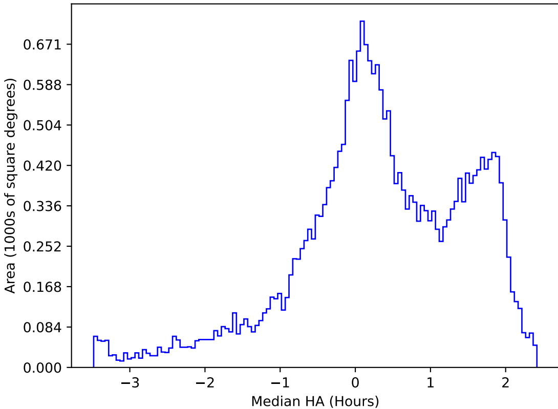
too_elab_r128_d3_gz_v3.4_10yrs All sky g band: Median HA
