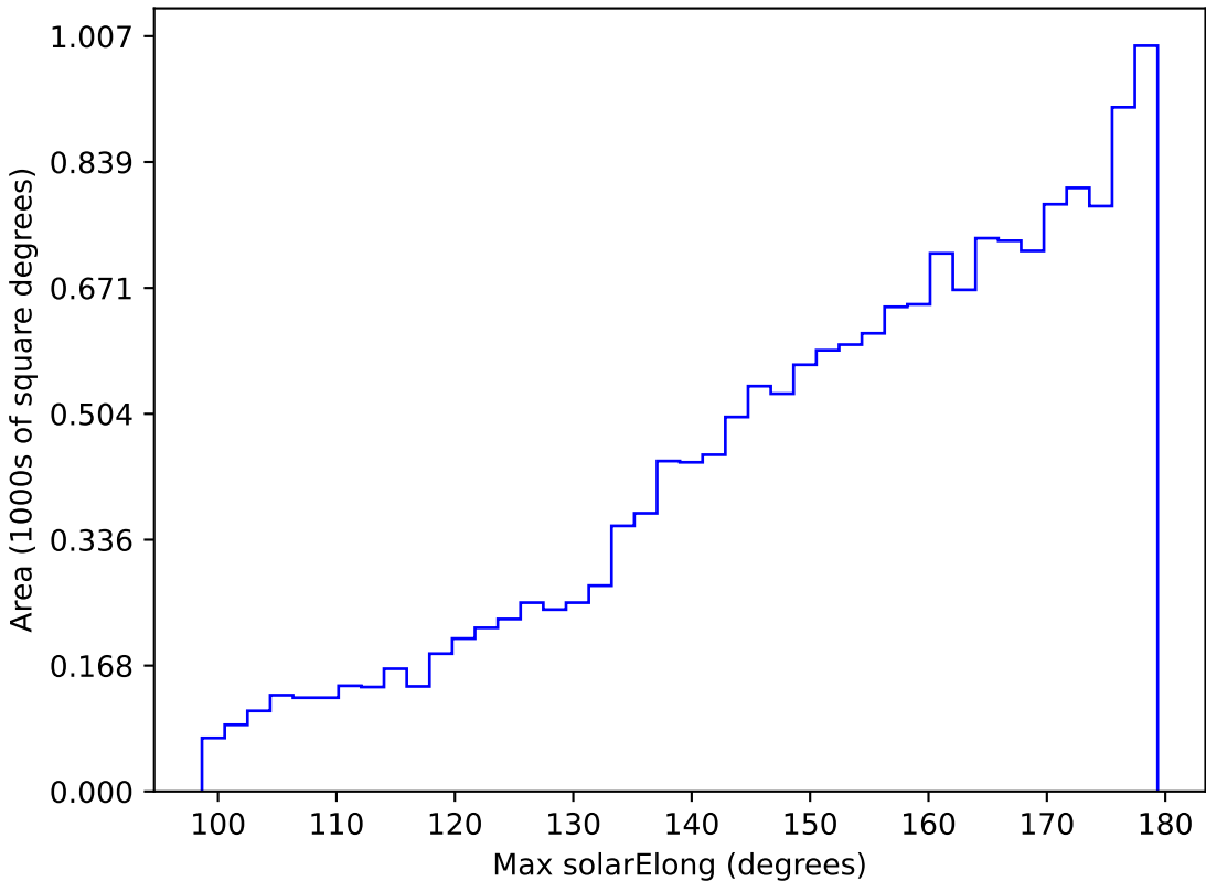
too_elab_r128_d3_gz_v3.4_10yrs WFD z band: Max solarElong
