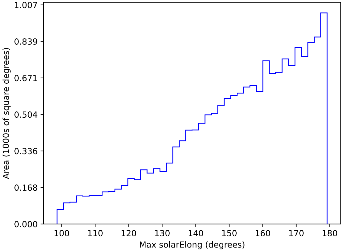
too_elab_r128_d3_gz_v3.4_10yrs WFD y band: Max solarElong
