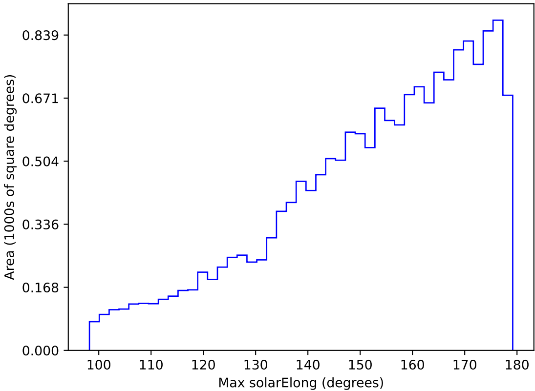
too_elab_r128_d3_gz_v3.4_10yrs WFD u band: Max solarElong
