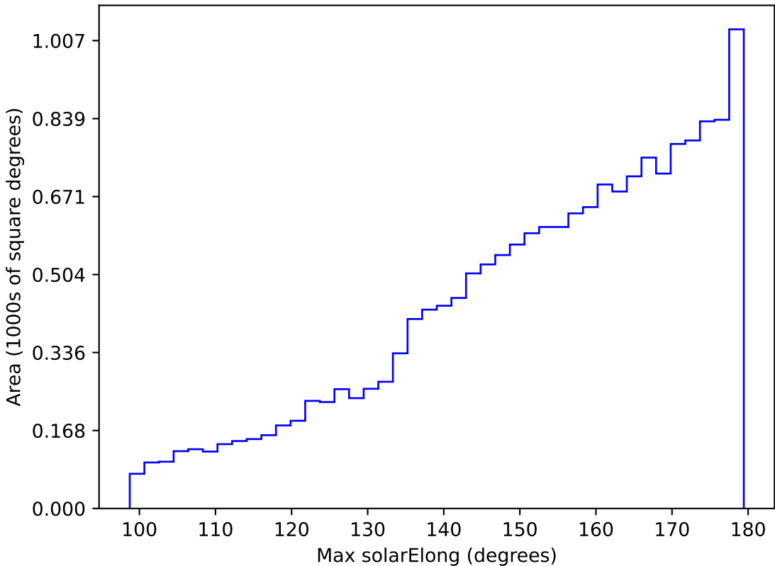
too_elab_r128_d3_gz_v3.4_10yrs WFD r band: Max solarElong
