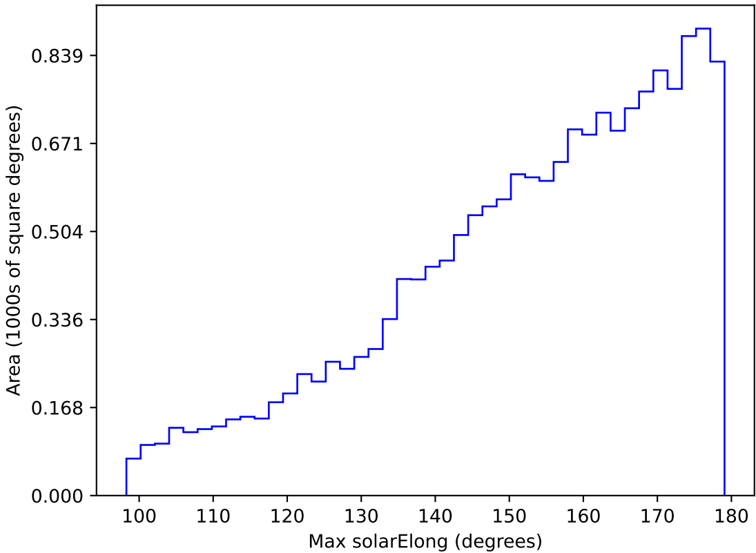
too_elab_r128_d3_gz_v3.4_10yrs WFD g band: Max solarElong
