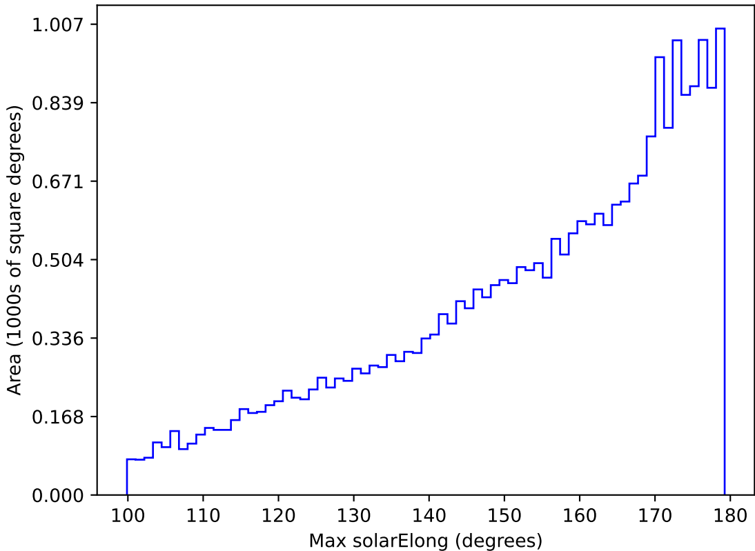
too_elab_r128_d3_gz_v3.4_10yrs All sky z band: Max solarElong
