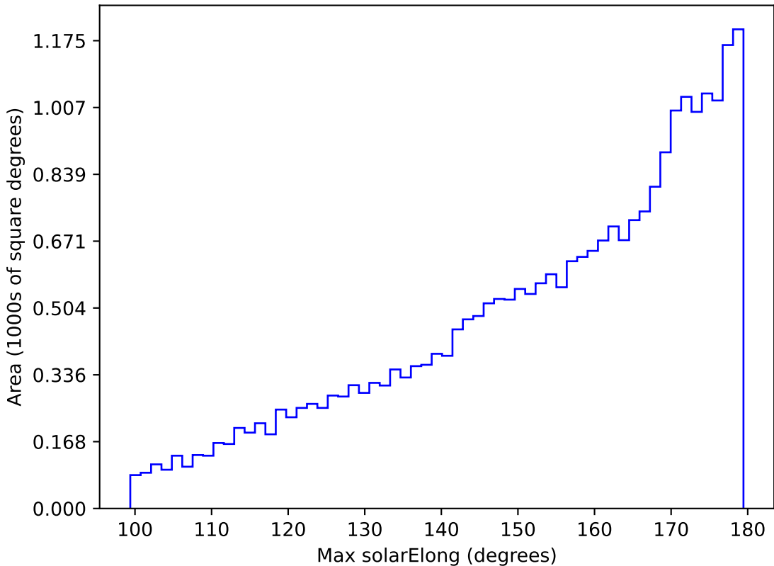
too_elab_r128_d3_gz_v3.4_10yrs All sky r band: Max solarElong
