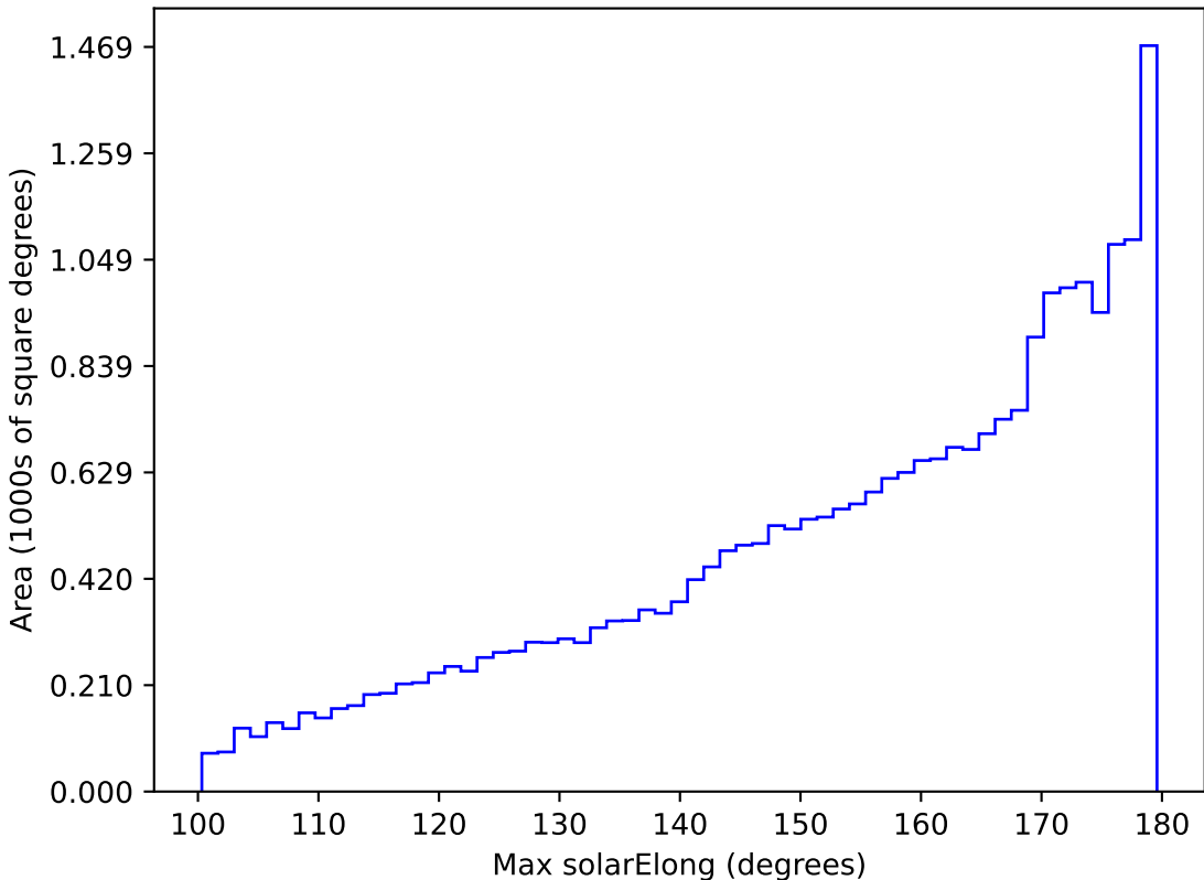
too_elab_r128_d3_gz_v3.4_10yrs All sky all bands: Max solarElong
