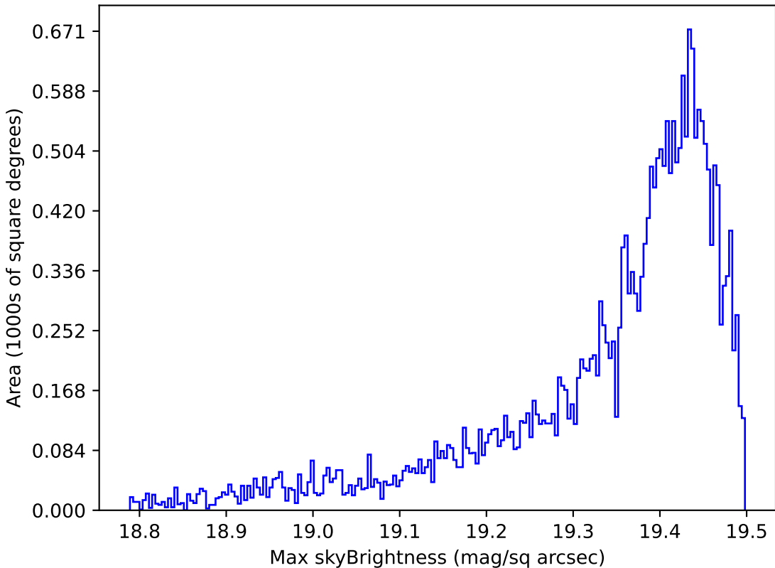
too_elab_r128_d3_gz_v3.4_10yrs Yr 1 z band: Max skyBrightness
