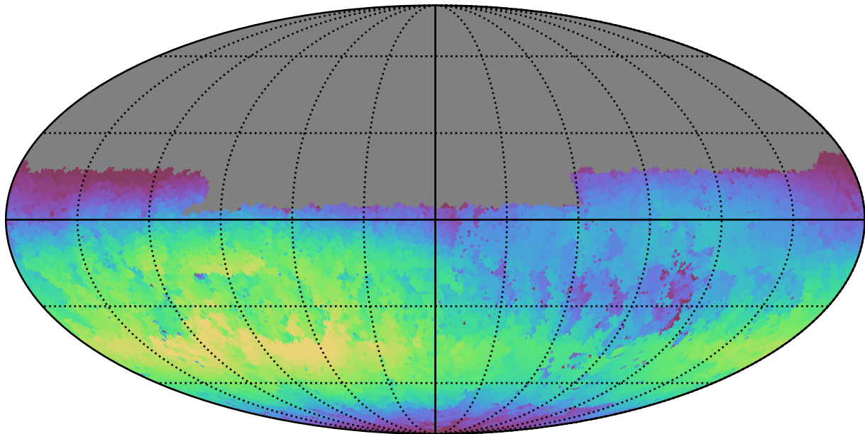
too_elab_r128_d3_gz_v3.4_10yrs Yr 1 u band: Max skyBrightness
