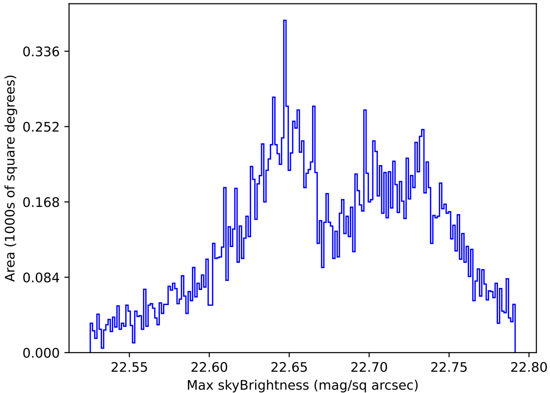
too_elab_r128_d3_gz_v3.4_10yrs Yr 1 u band: Max skyBrightness
