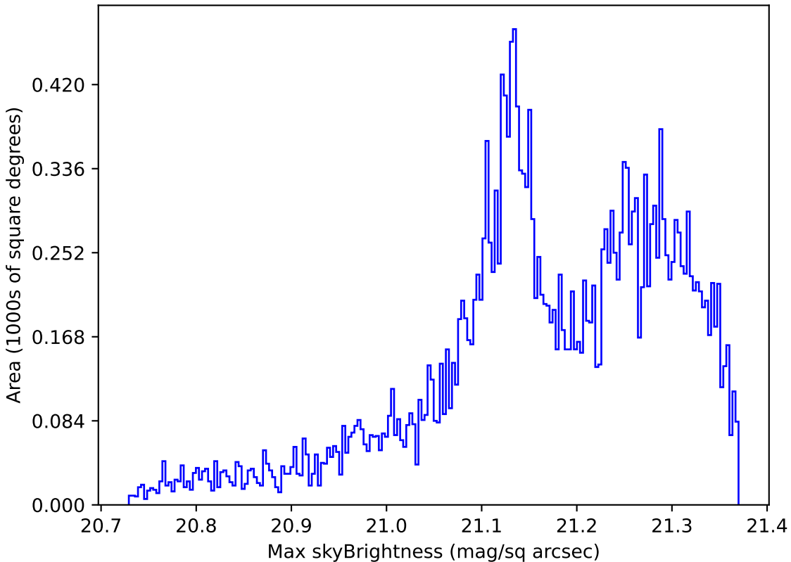
too_elab_r128_d3_gz_v3.4_10yrs Yr 1 r band: Max skyBrightness
