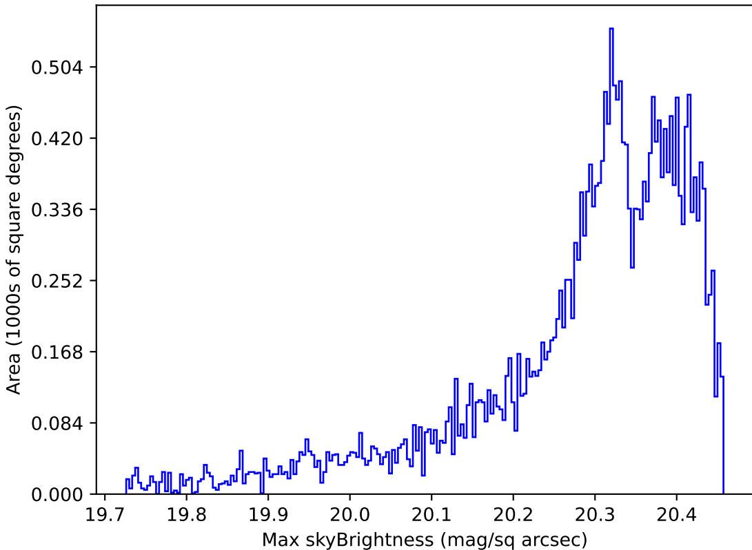
too_elab_r128_d3_gz_v3.4_10yrs Yr 1 i band: Max skyBrightness
