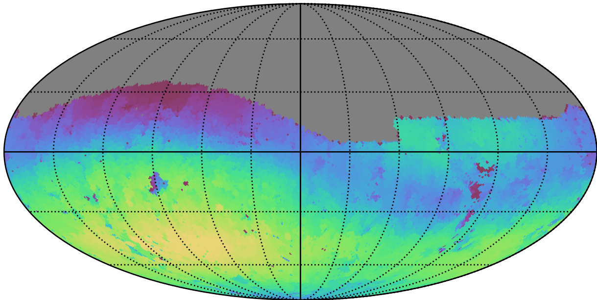
too_elab_r128_d3_gz_v3.4_10yrs Yr 1 g band: Max skyBrightness
