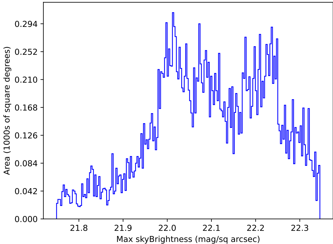
too_elab_r128_d3_gz_v3.4_10yrs Yr 1 g band: Max skyBrightness
