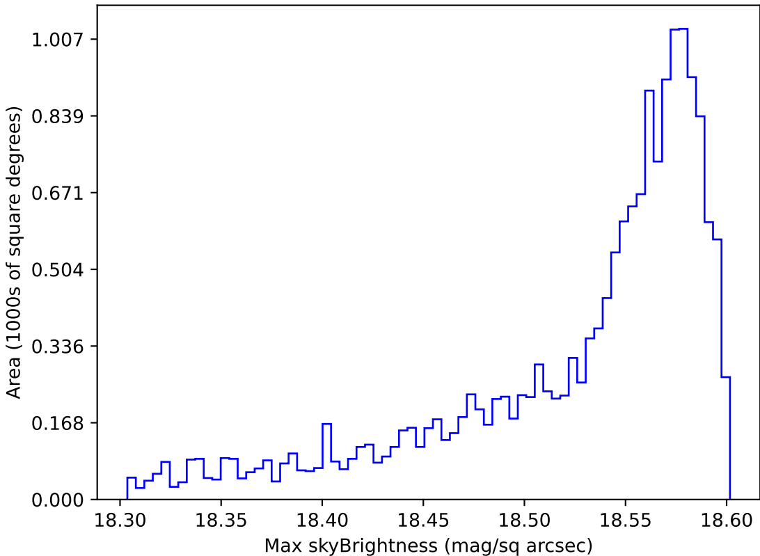
too_elab_r128_d3_gz_v3.4_10yrs WFD y band: Max skyBrightness
