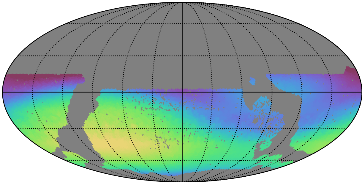
too_elab_r128_d3_gz_v3.4_10yrs WFD r band: Max skyBrightness
