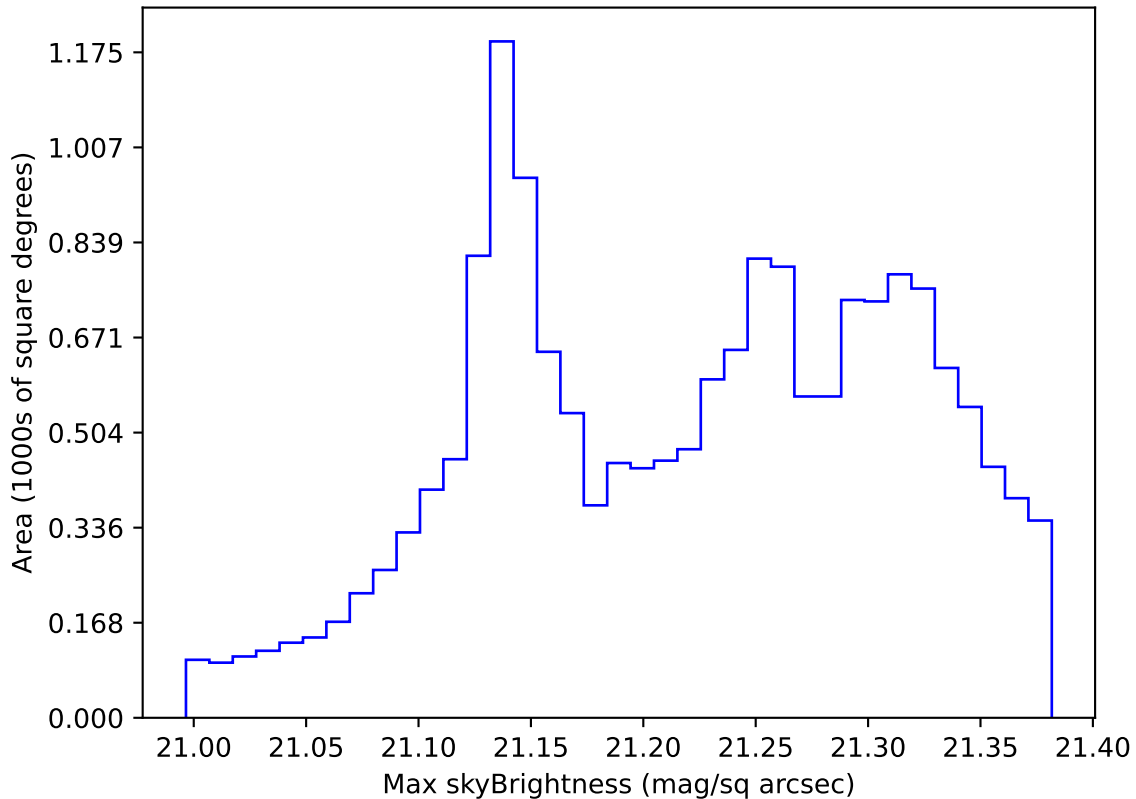
too_elab_r128_d3_gz_v3.4_10yrs WFD r band: Max skyBrightness
