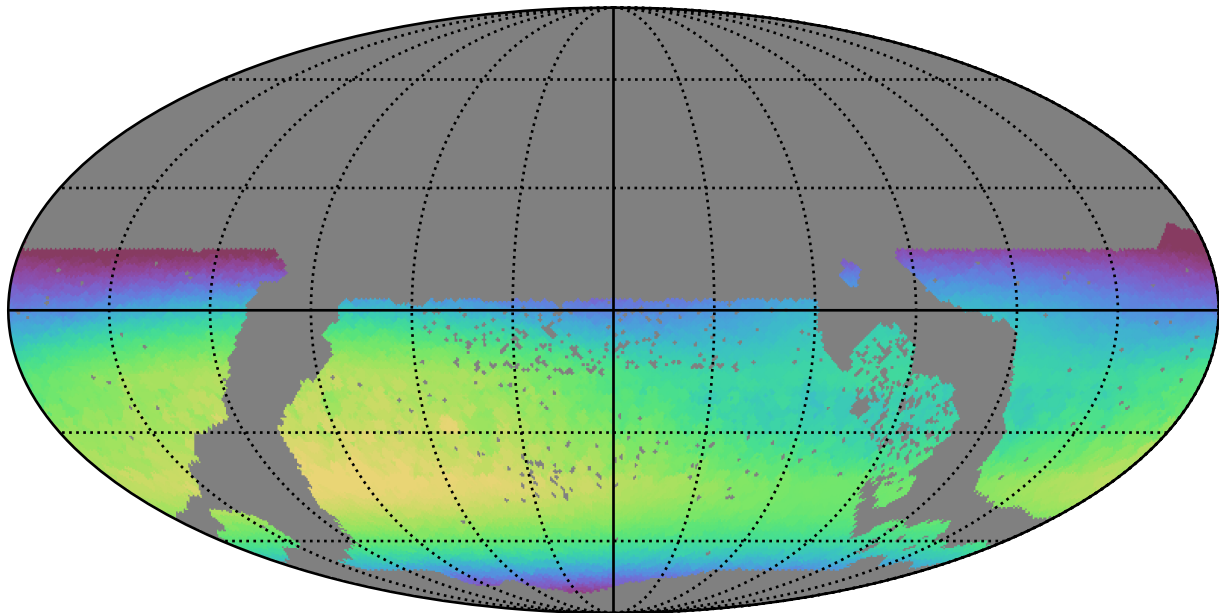
too_elab_r128_d3_gz_v3.4_10yrs WFD i band: Max skyBrightness
