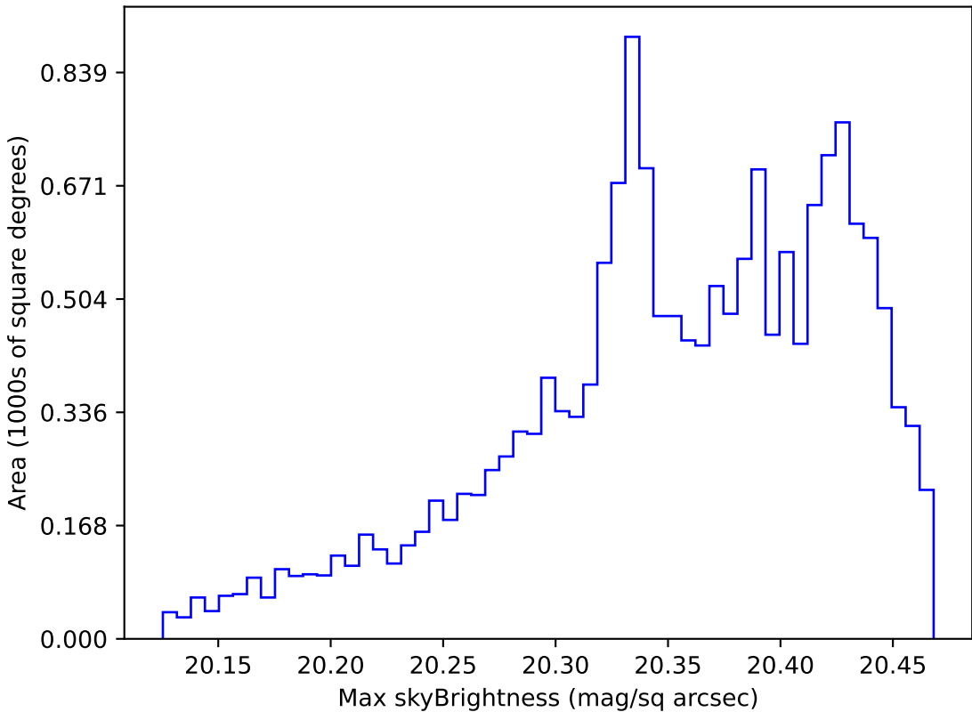
too_elab_r128_d3_gz_v3.4_10yrs WFD i band: Max skyBrightness
