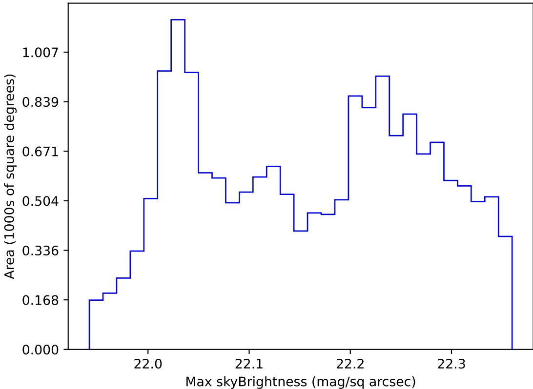
too_elab_r128_d3_gz_v3.4_10yrs WFD g band: Max skyBrightness
