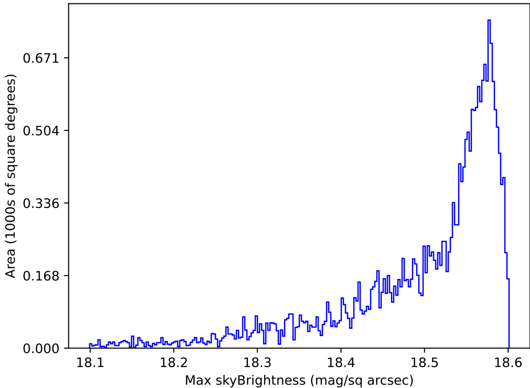
too_elab_r128_d3_gz_v3.4_10yrs All sky y band: Max skyBrightness
