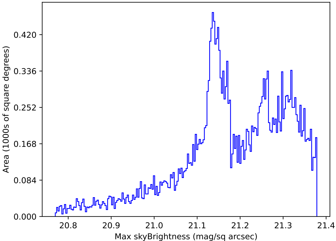
too_elab_r128_d3_gz_v3.4_10yrs All sky r band: Max skyBrightness
