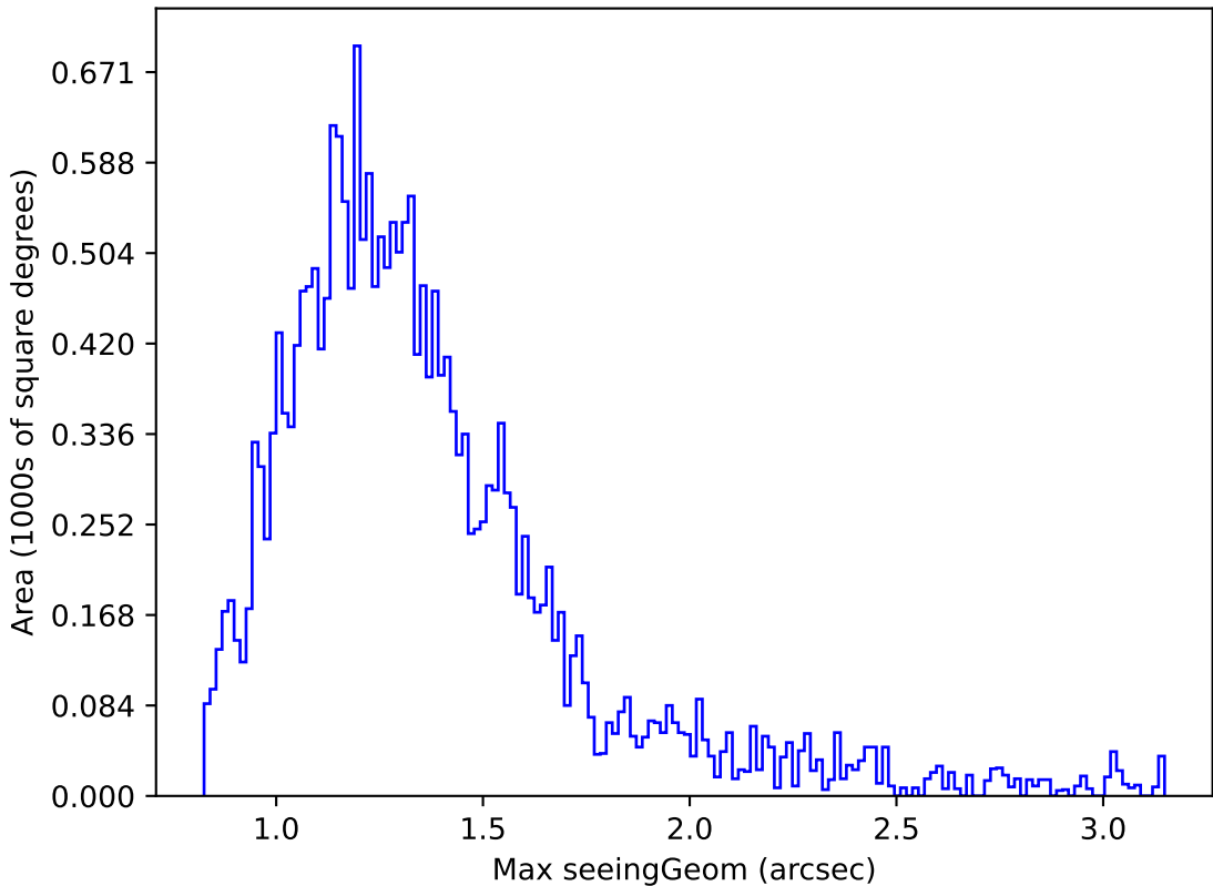
too_elab_r128_d3_gz_v3.4_10yrs Yr 1 u band: Max seeingGeom
