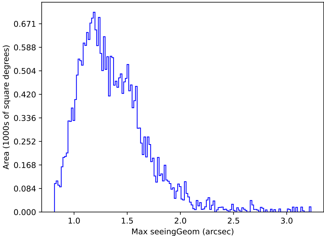
too_elab_r128_d3_gz_v3.4_10yrs Yr 1 r band: Max seeingGeom
