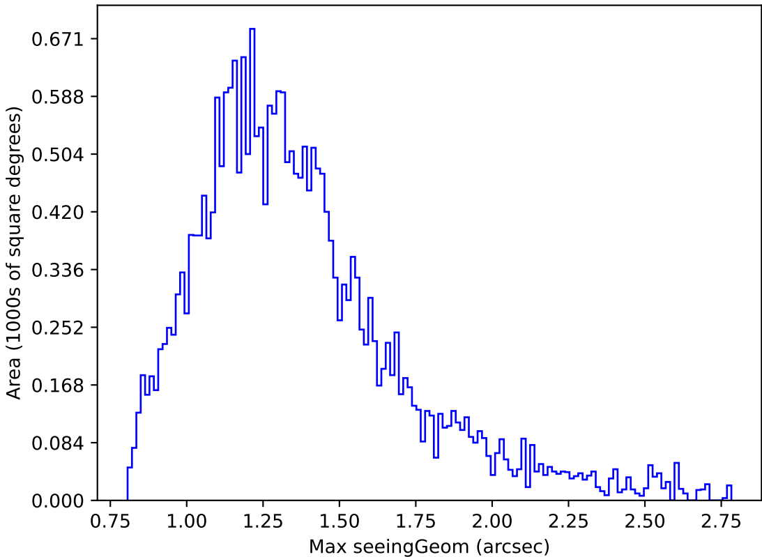
too_elab_r128_d3_gz_v3.4_10yrs Yr 1 i band: Max seeingGeom
