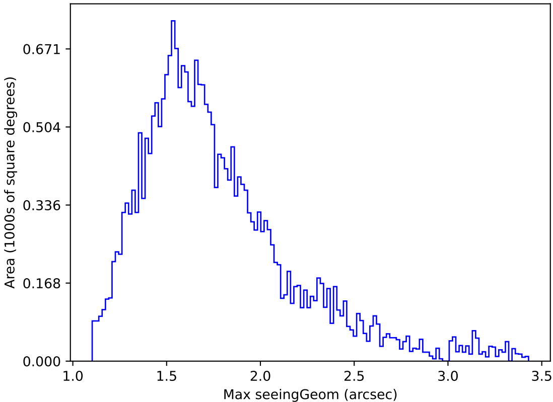
too_elab_r128_d3_gz_v3.4_10yrs Yr 1 all bands: Max seeingGeom
