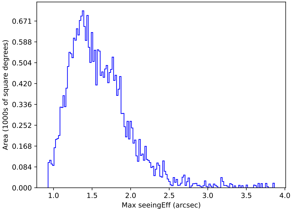
too_elab_r128_d3_gz_v3.4_10yrs Yr 1 r band: Max seeingEff
