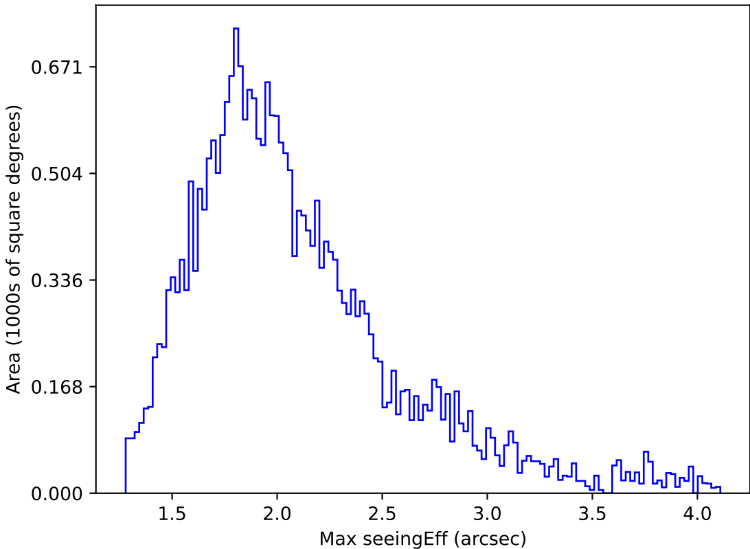
too_elab_r128_d3_gz_v3.4_10yrs Yr 1 all bands: Max seeingEff
