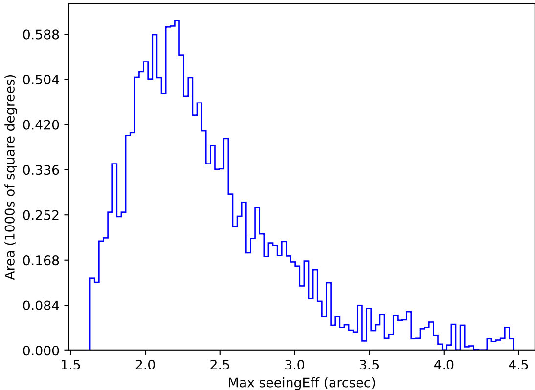
too_elab_r128_d3_gz_v3.4_10yrs WFD y band: Max seeingEff
