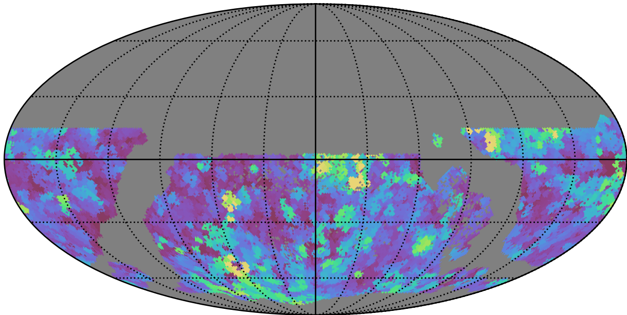
too_elab_r128_d3_gz_v3.4_10yrs WFD g band: Max seeingEff
